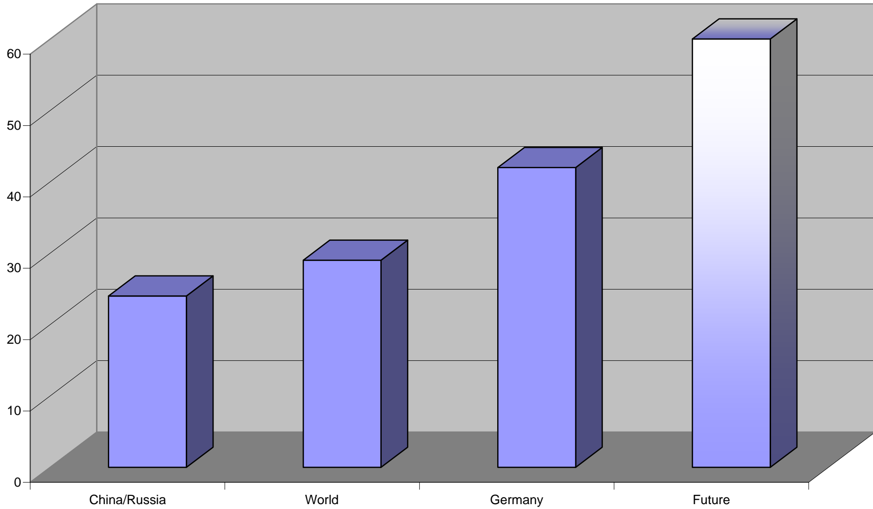
Comparison of the efficiency of international power plants using hard coal (efficiency indicated in %)
